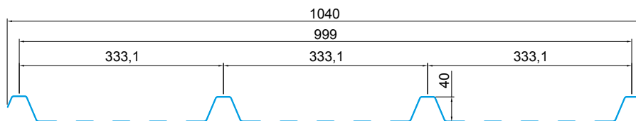
TOPLIGHT T 333/45 compatible with "REX 45.333.1000"
