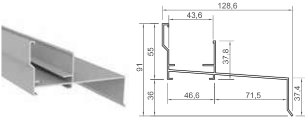
ALUMINIUM LOWER PROFILE WITH SILL
