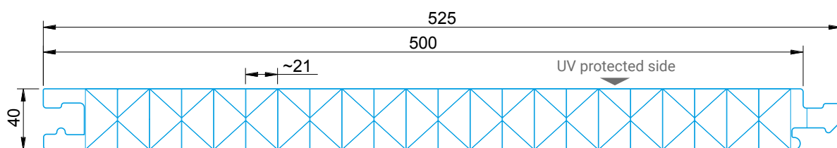
Wall 500-40 mono X
