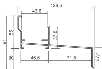
LOWER ALUMINIUM PROFILE WITH SILL
