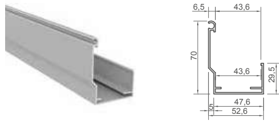
ALUMINIUM LOWER PROFILE
